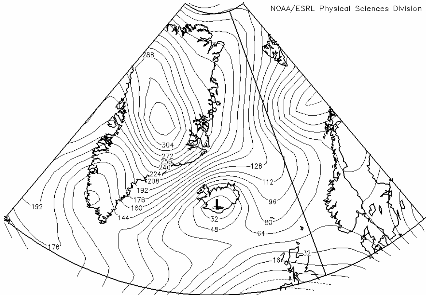
1000mb Geopotential Heights (m) Composite Mean 4/9/1963 18z 20thC Reanalysis V2
